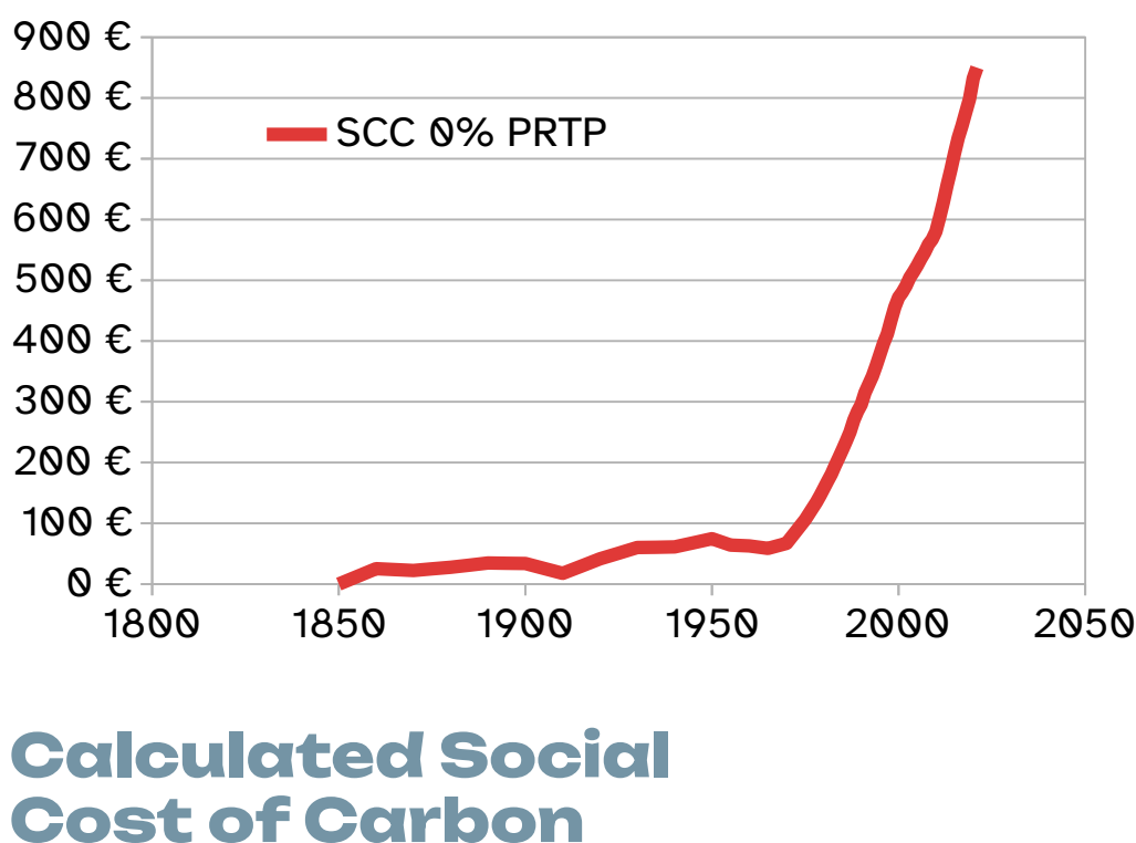
Figure 1: Calculated Social Cost of Carbon
